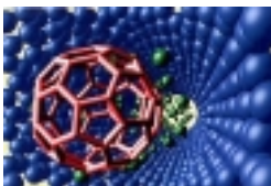
Buckminsterfullerene
