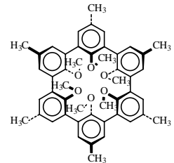
Spherand
